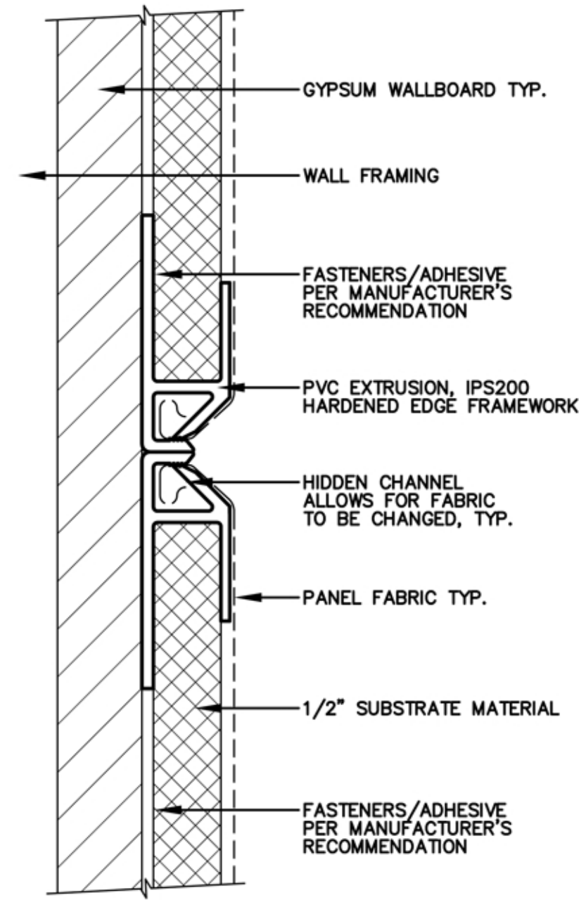
2 IPS200 1/2" BEVELED EDGE BUTT JOINT FULL
