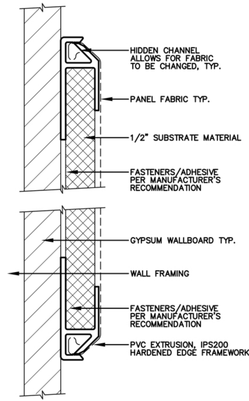
1 IPS200 1/2" BEVELED EDGE FREESTANDING FULL
