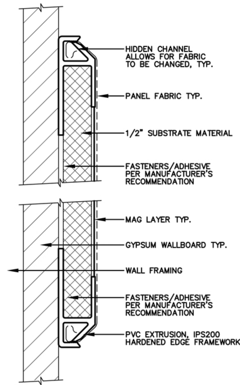
5 IPS200 1/2" BEVELED MAG-TACK REVERSE FOR SQUARE EDGE FULL
