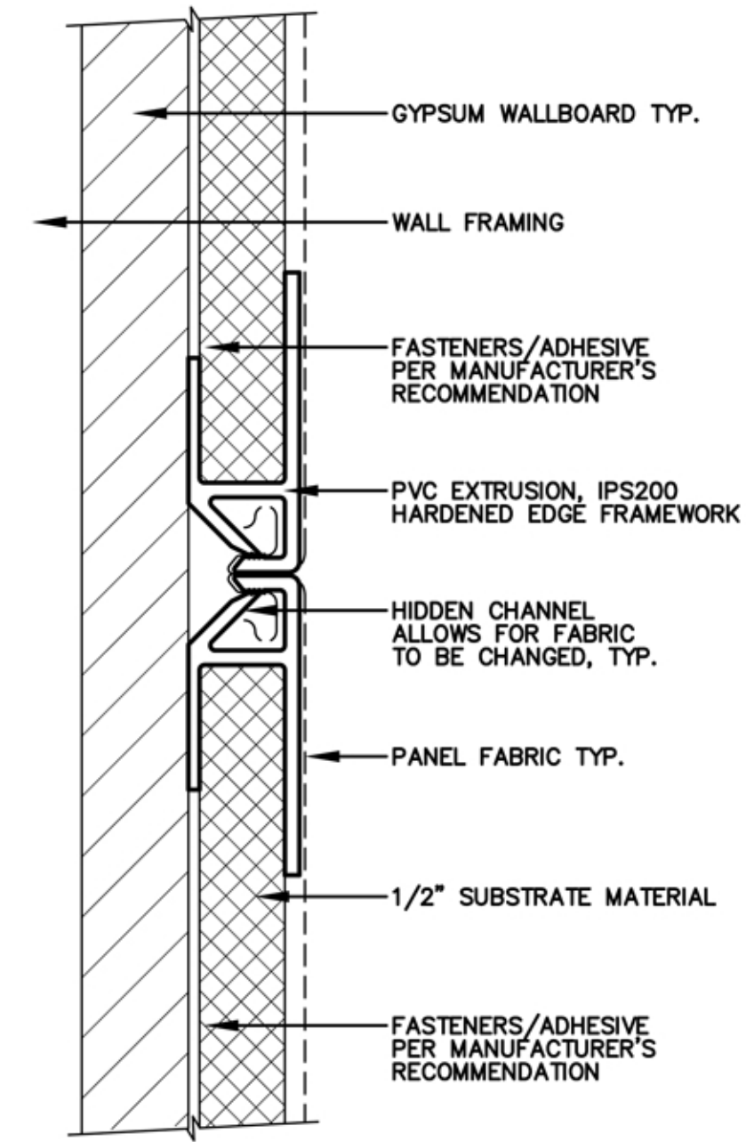
3 IPS200 1/2" SQUARE EDGE BUTT JOINT FULL
