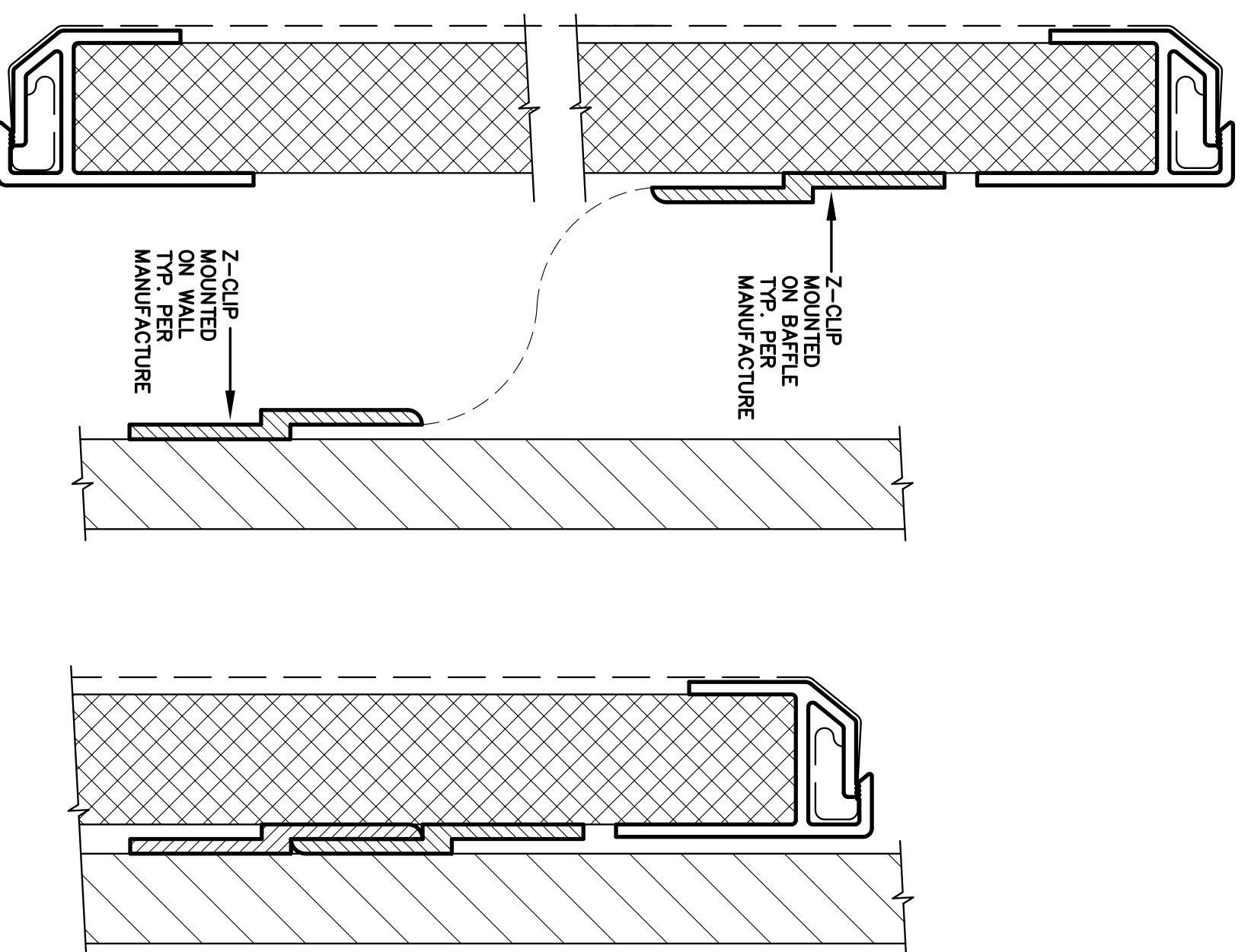
10 FULL IPS250 Z-CLIP MOUNT
