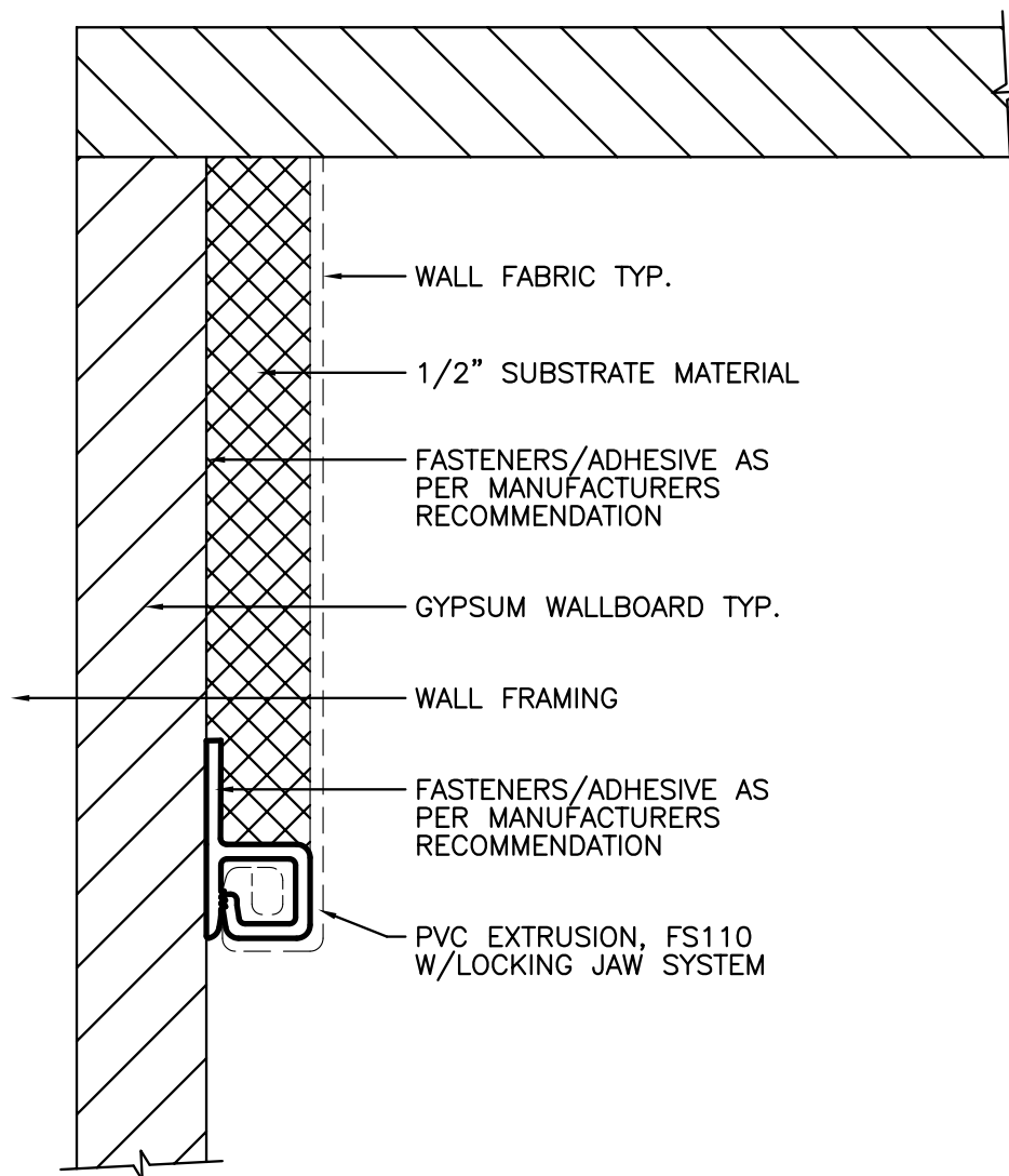
21 FS110 FREESTANDING PANEL EDGE FULL
