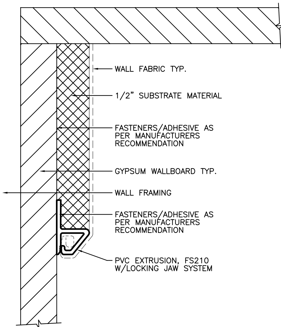
22 FS210 FREESTANDING PANEL EDGE FULL
