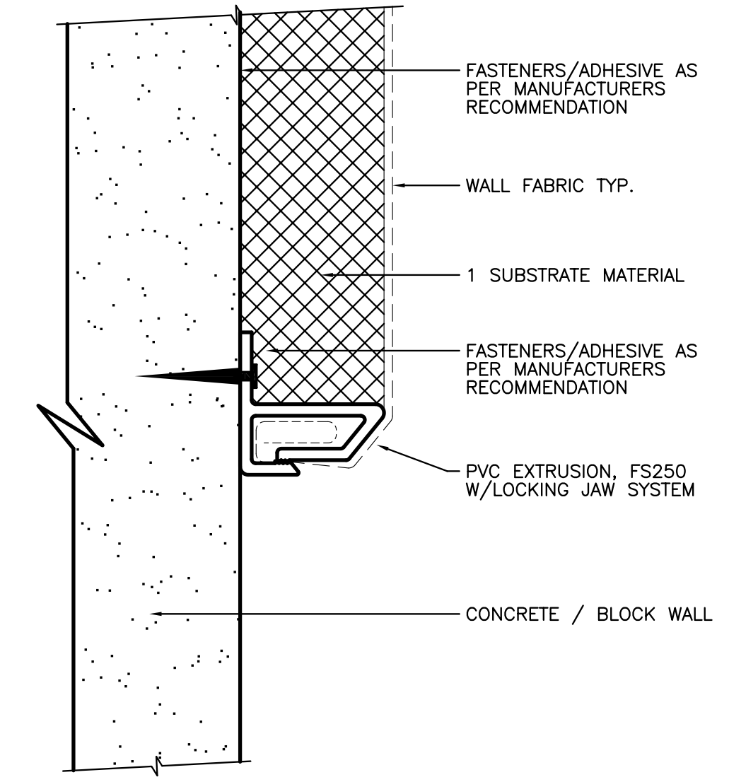
20 FS250 CONCRETE FASTENING FULL
