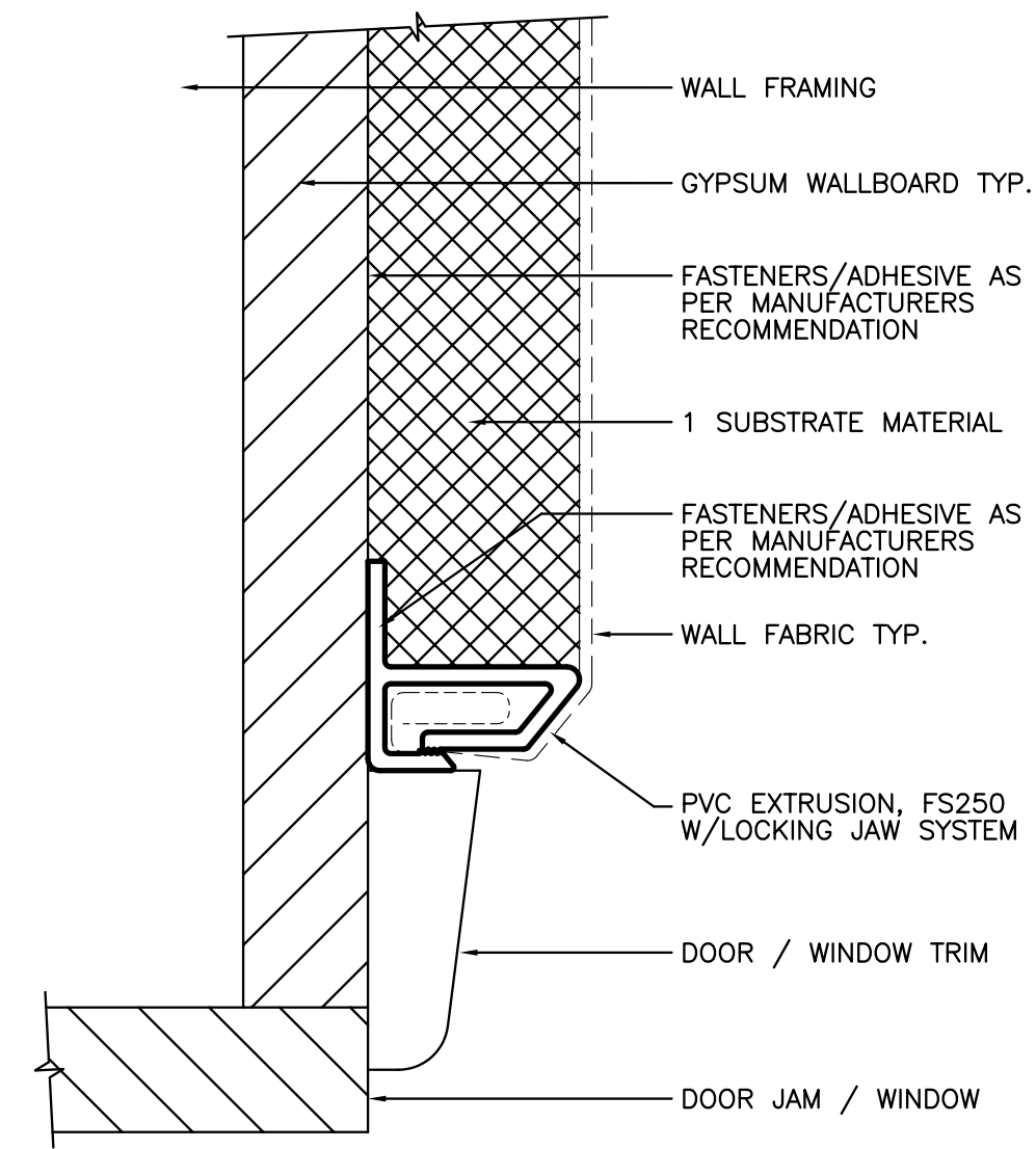
18 FS250 DOORS / WINDOWS FULL
