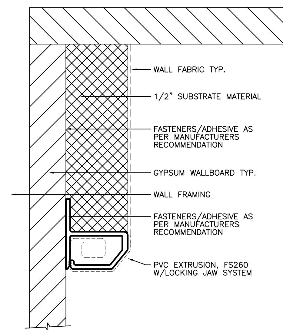
22 FS260 FREESTANDING PANEL EDGE FULL
