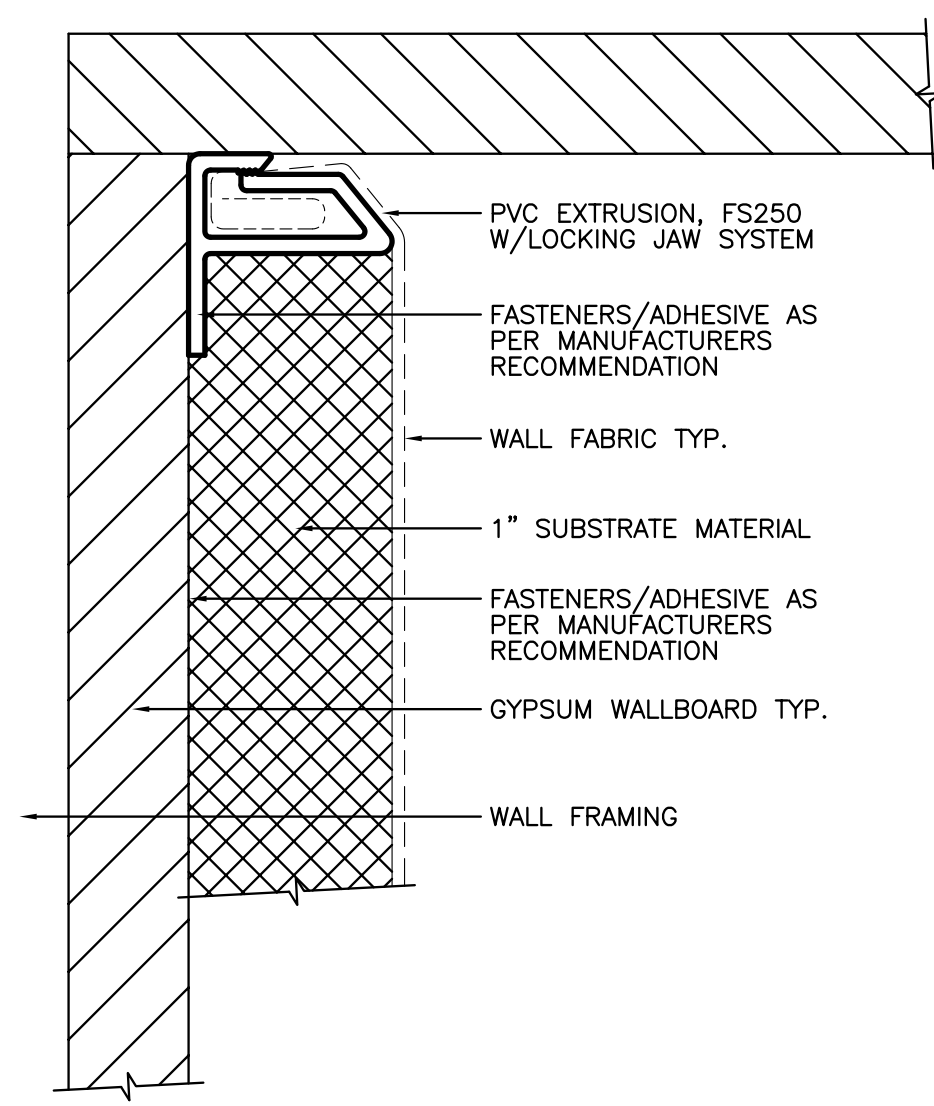
17 FS250 CEILINGS / SOFFITS FULL
