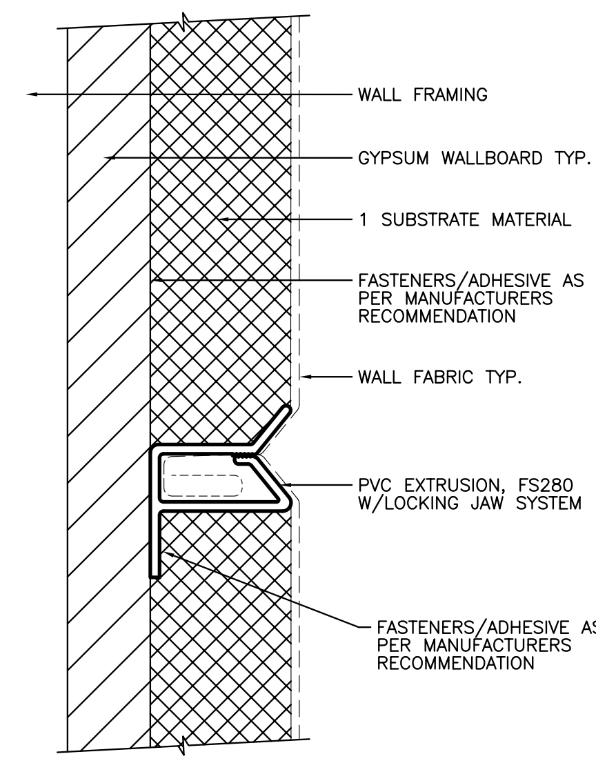
19 FS280 INTERMEDIATE JOINT FULL
