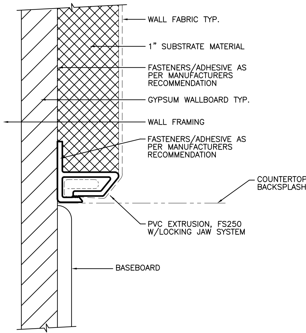
16 FS250 BASE / COUNTERTOPS FULL
