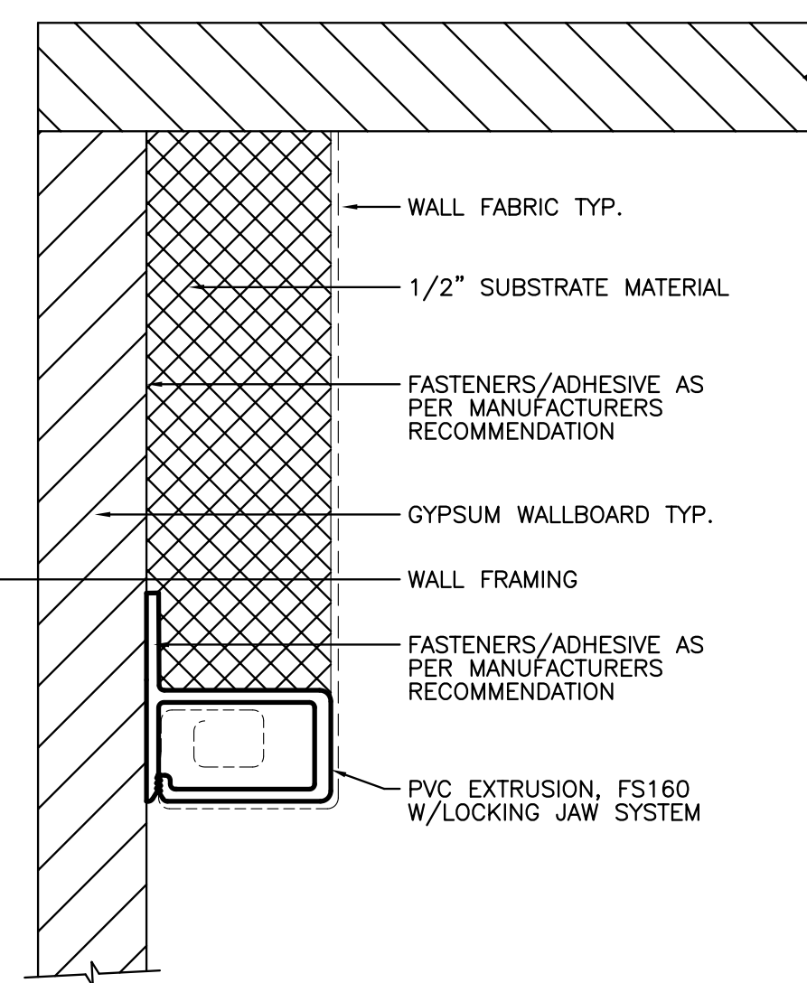
22 FS160 FREESTANDING PANEL EDGE FULL
