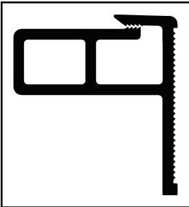
FS155 Profile (Actual Size)
