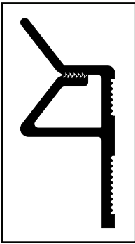
FS230 Profile (Actual Size)
