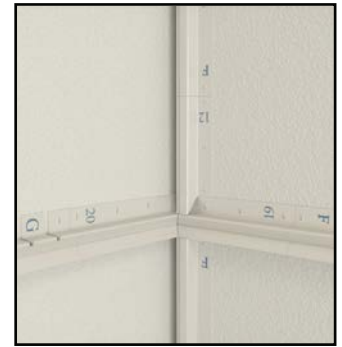
Inside Corner Cross Seam with FS230
